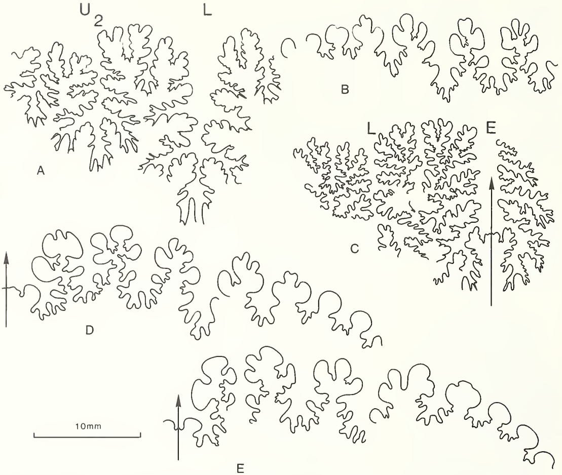
TEXT-FIG. 6. Sutures of A, Pachydiscus (Pachydiscus) neubergicus neubergicus (Hauer, 1858), the lectotype of Anmonites chrishna , Forbes, 1846, BMNH C51041. B, D, E, Sphenodiscus siva (Forbes, 1846). B, D, BMNH C51088, E, BMNH C51087. C, Menuites menu (Forbes, 1846), BMNH C47550.
